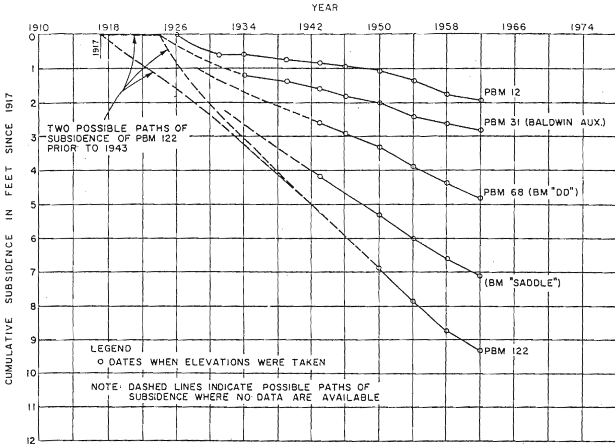
Figure 10 SUBSIDENCE OF BENCH MARKS BALDWIN HILLS AREA
